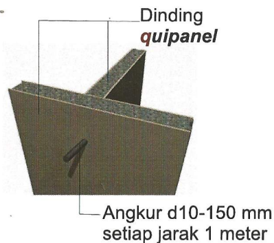
Detail sambungan Panel T
